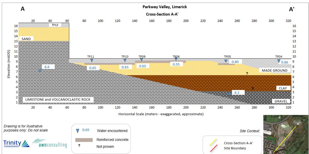
Figure 5-10: Cross-Section A-A'
