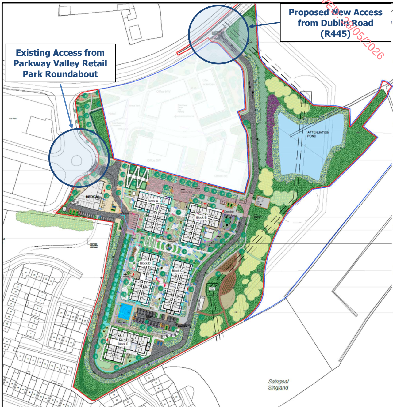
Figure 2-5 Site Layout Plan showing Proposed Site Access Locations (Source: Site Plan is Extract from Landscape Plan Drawing PAV-JBA-XX-XX-DR-L-0002, JBA, May 2026)
